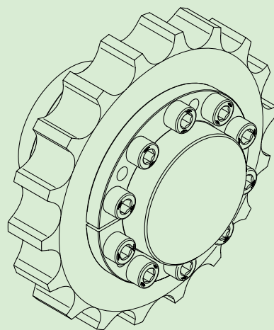
Pinion gear connection
