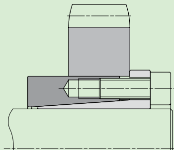
Pinion gear connection
