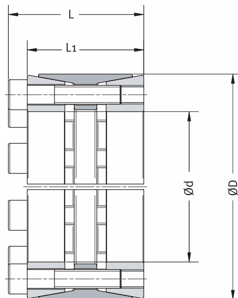
Example of order: MAV 1008 100 x 145
