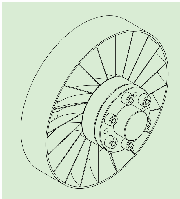
Connection of fan with thin walled hub
