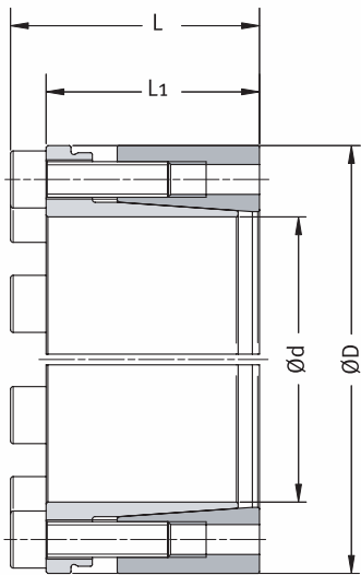
Example of order: MAV 6901 50 x 80
